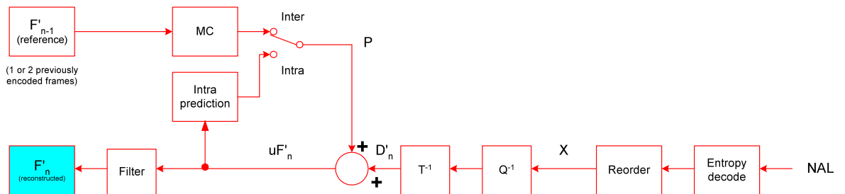
Figure 2-2 AVC Decoder
