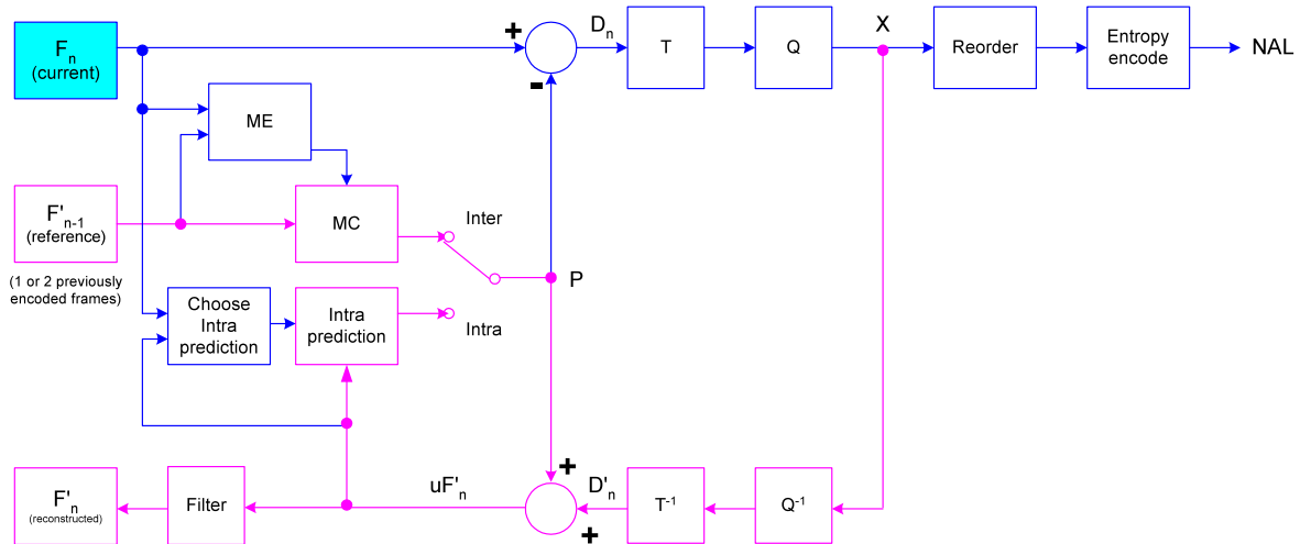
Figure 2-1 AVC Encoder
